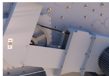
SEGMENTED BELT GUARD
